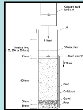
Fig 3. Experimental ISSF schematic
