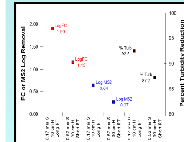
Fig 7. Comparison of mean performance of ISSF best and worst design and operating factor combinations.
