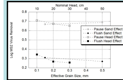
Fig 5. Mean log MS2 coliphage removal by factor level for long (Pause) and short (Flush) RT.
