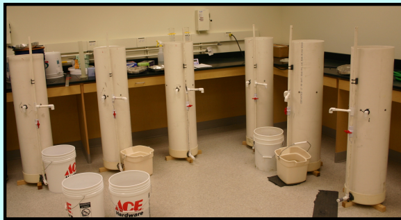
Fig 2. Intermittent slow sand filters fabricated for lab testing.
